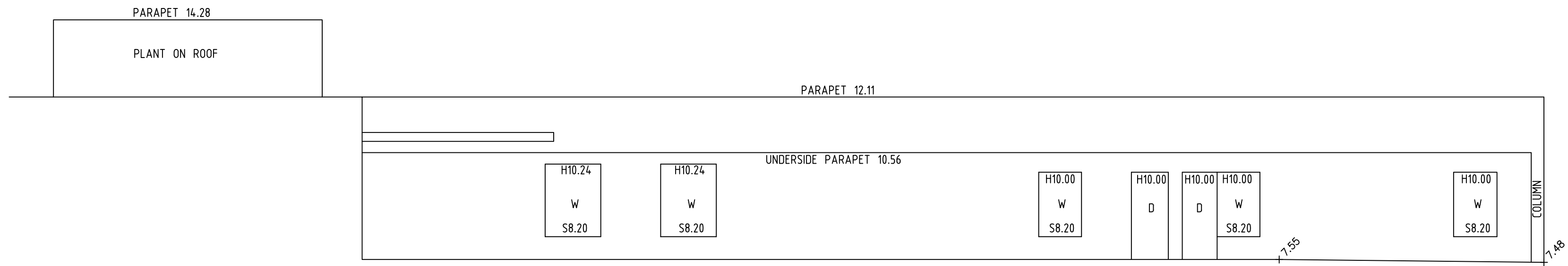
JARA WARD BUILDING No 112) EASTERN ELEVATION
