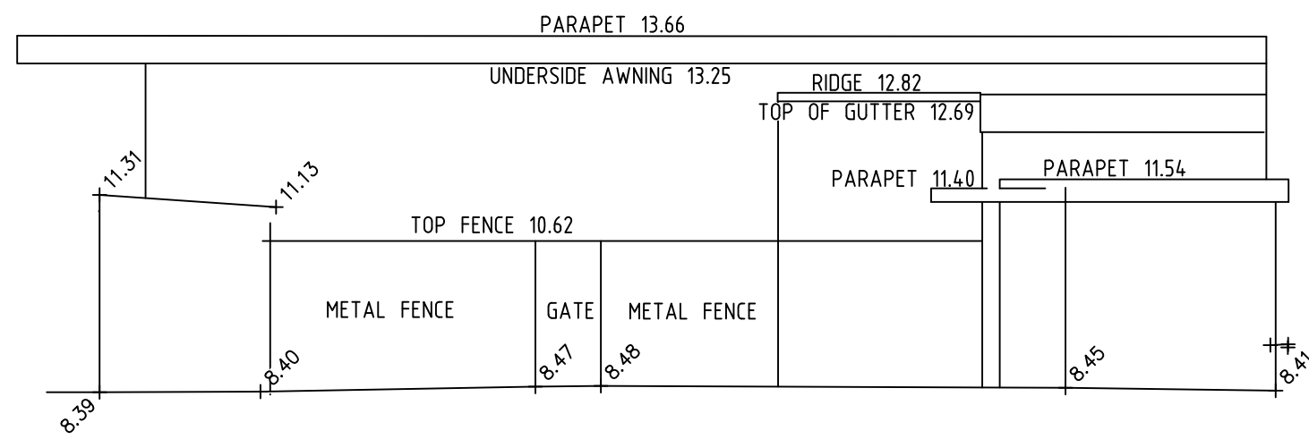
BUILDING No 28 SOUTHERN ELEVATION
