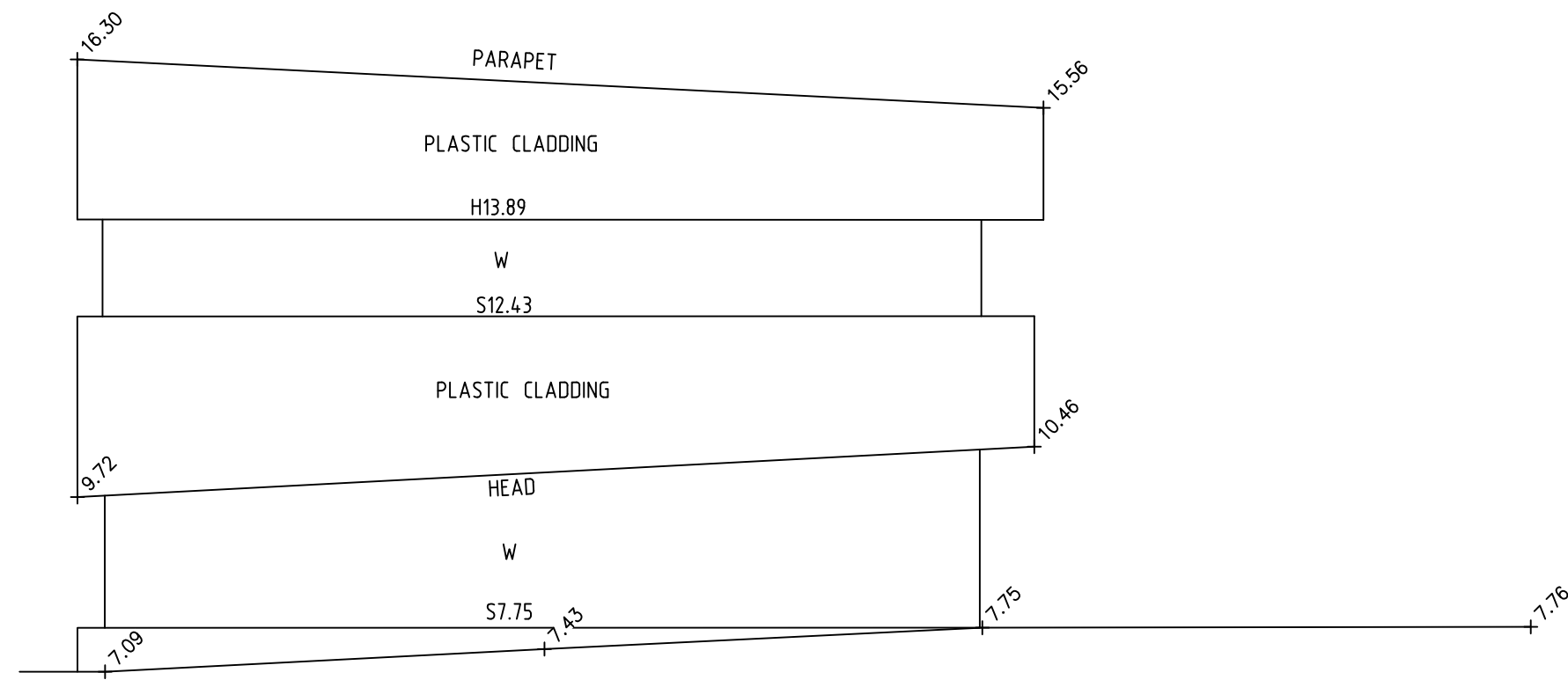
CONCORD MEDICAL EDUCATION CENTRE EASTERN ELEVATION
